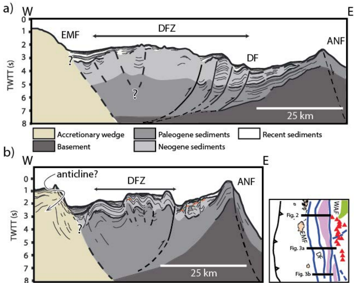
Figure 3. Structural interpretation of seismic sections in the Andaman showing backthrusting in the DF (Diligent Fault), anticline in the EMF (Eastern Margin Fault), and ANF (Andaman Nicobar Fault) to the south of Andaman Spreading Center (ASC). Modified after Moeremans and Singh (2015). ANF is equivalent to WAF (West Andaman Fault) of Curray (2005). DFZ (Diligent Fault Zone) is dominated by thrust faults and folded sediments.
